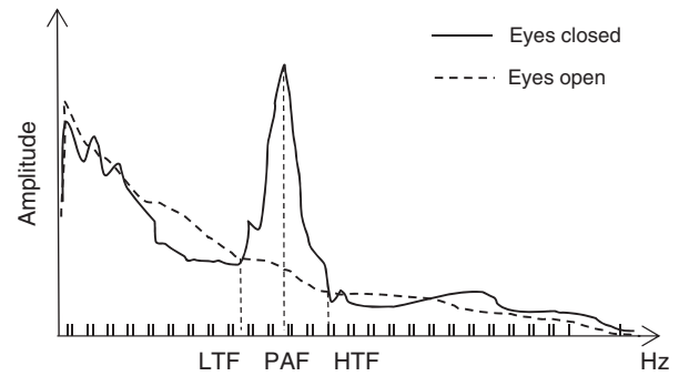
Fig. 1. The demonstration of individual alpha band. (individual alpha band: LTF–HTF, individual lower alpha band: LTF–PAF, individual upper alpha band: PAF–HTF).
