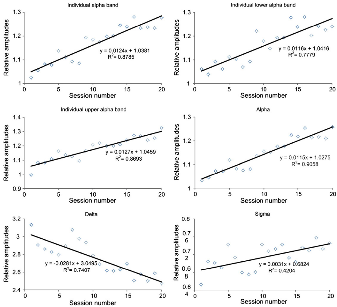
Fig. 2. The average relative amplitudes in the examined bands of all subjects over training sessions. The straight line results from a linear regression and indicates a linear sustained change.
